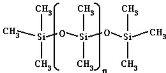
Polydimethylsiloxane
